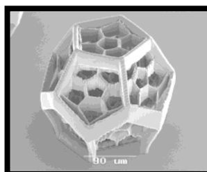
Fig. 2: 3-D structure fabricated from hybrid sol-gel materials
